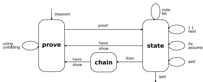
Figure 2.3: Isar/VM modes
