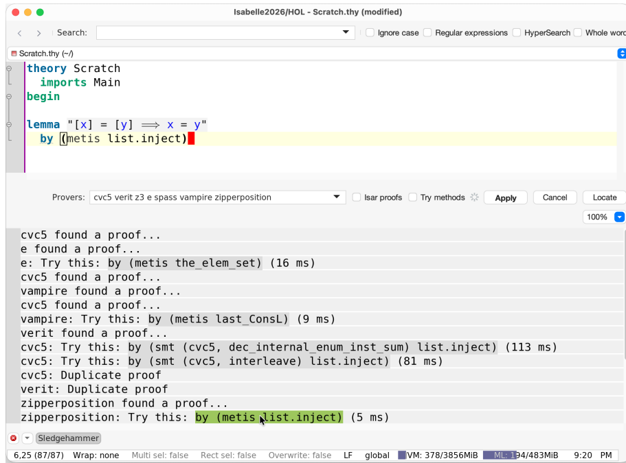
Figure 3.13: An instance of the Sledgehammer panel
