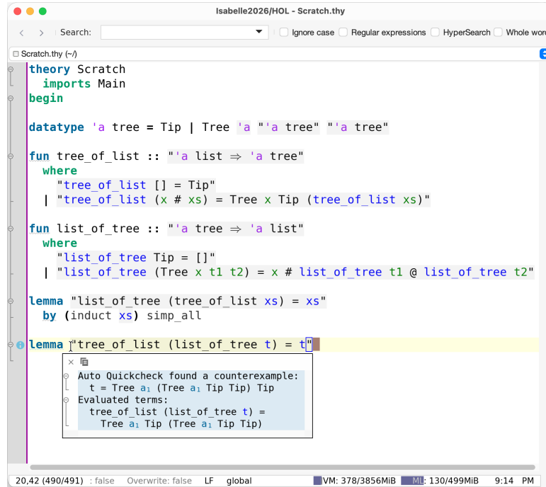
Figure 3.12: Result of automatically tried tools
