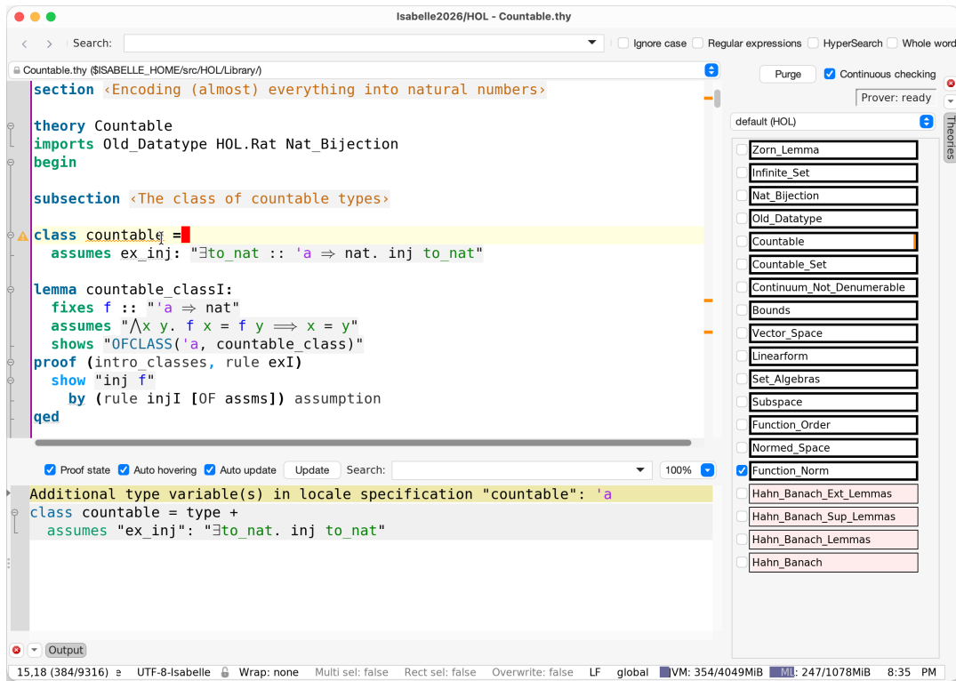
Figure 3.2: Multiple views on prover output: gutter with icon, text area with popup, text overview column, Theories panel, Output panel
