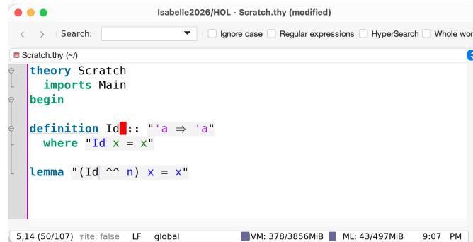
Figure 3.11: The result of semantic selection and systematic renaming
