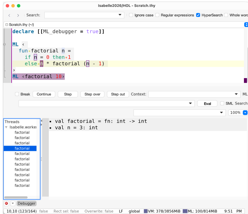
Figure 5.1: ML debugger session
