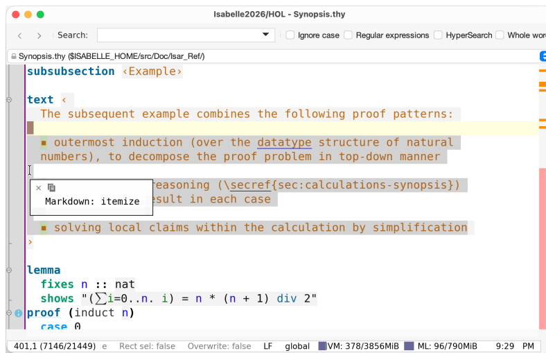
Figure 4.2: Markdown structure within document text
