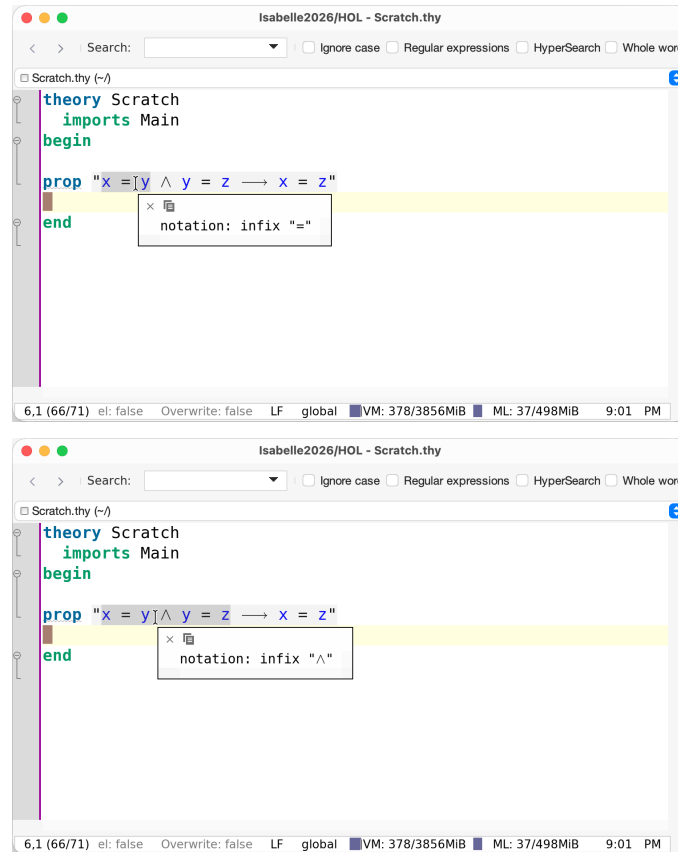
Figure 3.9: Visualized markup for nested infix expressions
