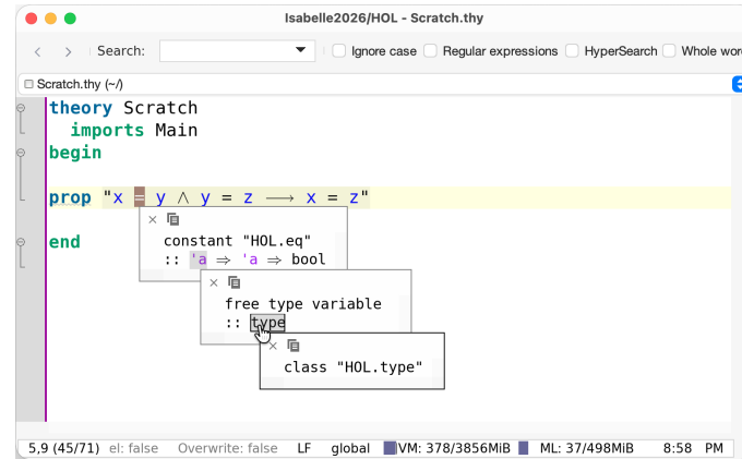
Figure 3.8: Nested tooltips over formal entities
