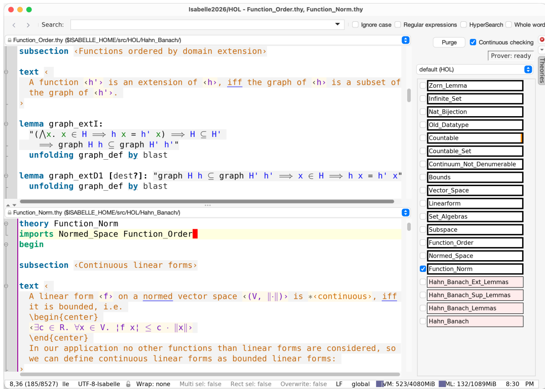
Figure 3.1: Theories panel with an overview of the document-model, and jEdit text areas as editable views on some of the document nodes
