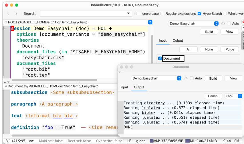
Figure 4.5: Document panel with separate instances for Input and Output
