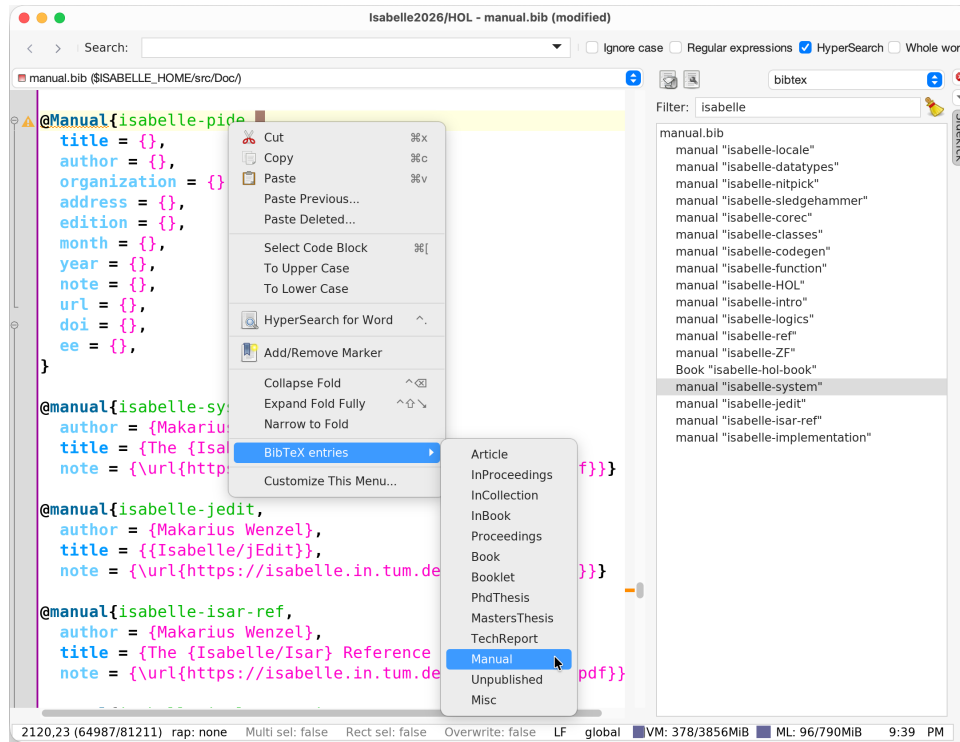
Figure 4.4: BibT E X mode with context menu, SideKick tree view, and semantic output from the bibtex tool
