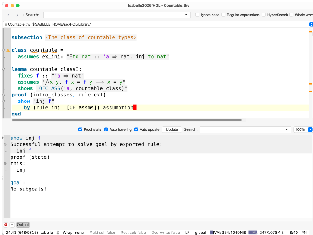
Figure 3.3: Proof state display within the regular output panel
