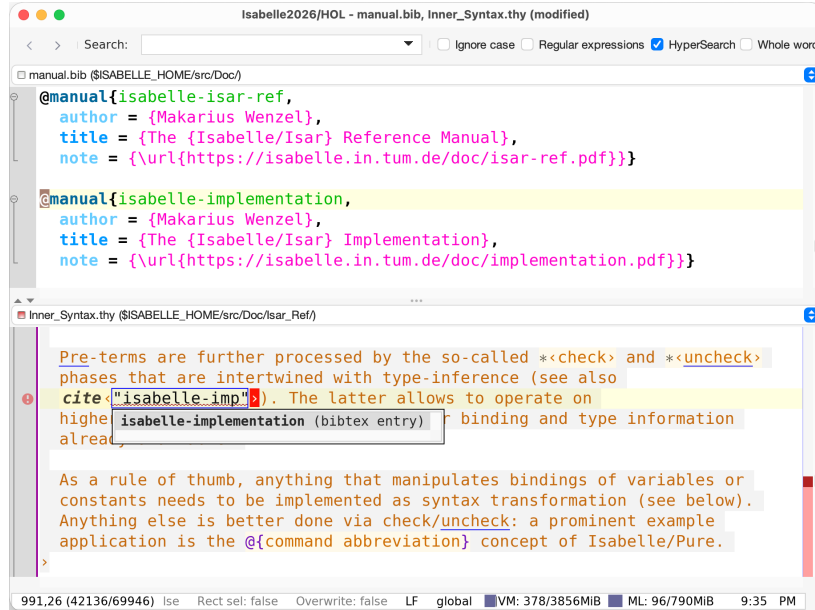
Figure 4.3: Semantic completion of citations from open BibTeX files
