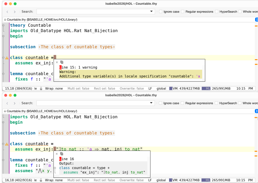
Figure 3.4: Line status output via keyboard shortcut CS+1
