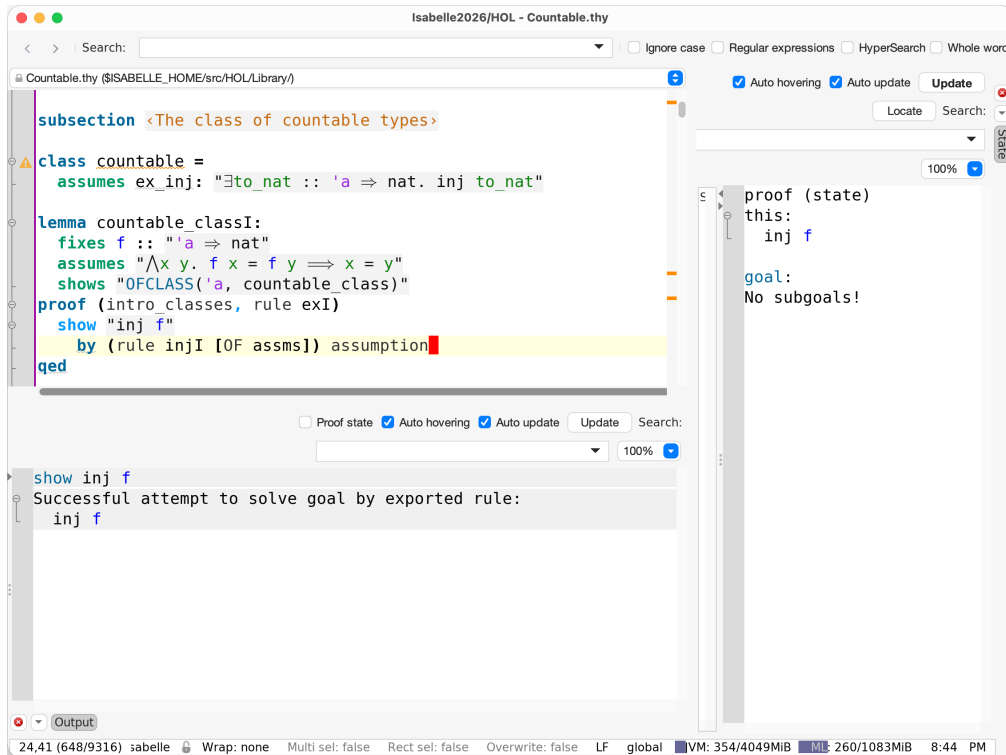
Figure 3.5: Separate proof state display (right) and other output (bottom).
