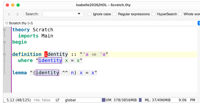
Figure 3.10: Scope of formal entity: defining vs. referencing positions
