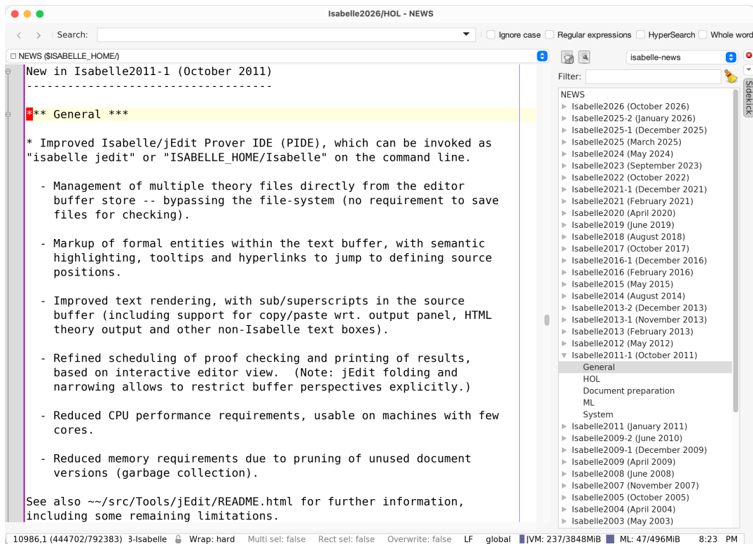
Figure 2.1: The Isabelle NEWS file with SideKick tree view
