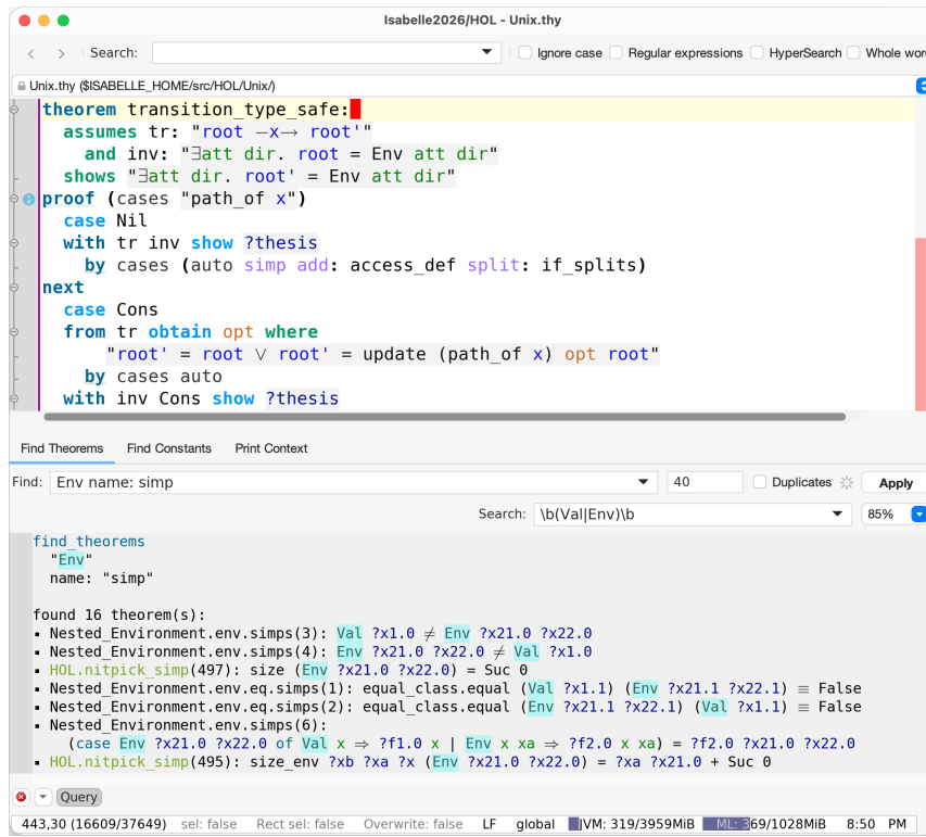
Figure 3.6: An instance of the Query panel: find theorems
