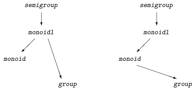
Fig. 8.1. Subclass relationship of monoids and groups: before and after establishing the relationship \text{group} \subseteq \text{monoid} ; transitive edges are left out.
